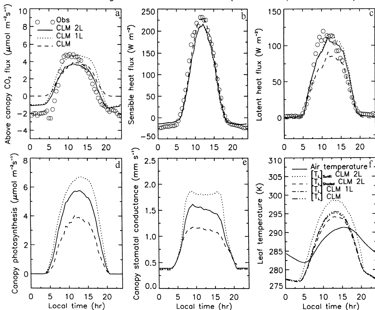
FIG. 8. Same as in Fig. 6 except over old black spruce at BOREAS/NOBS research site (1 Jun–30 Sep 1994). Also, the model averages are based on the time step values that are sampled only for the time step in which observation were taken.
